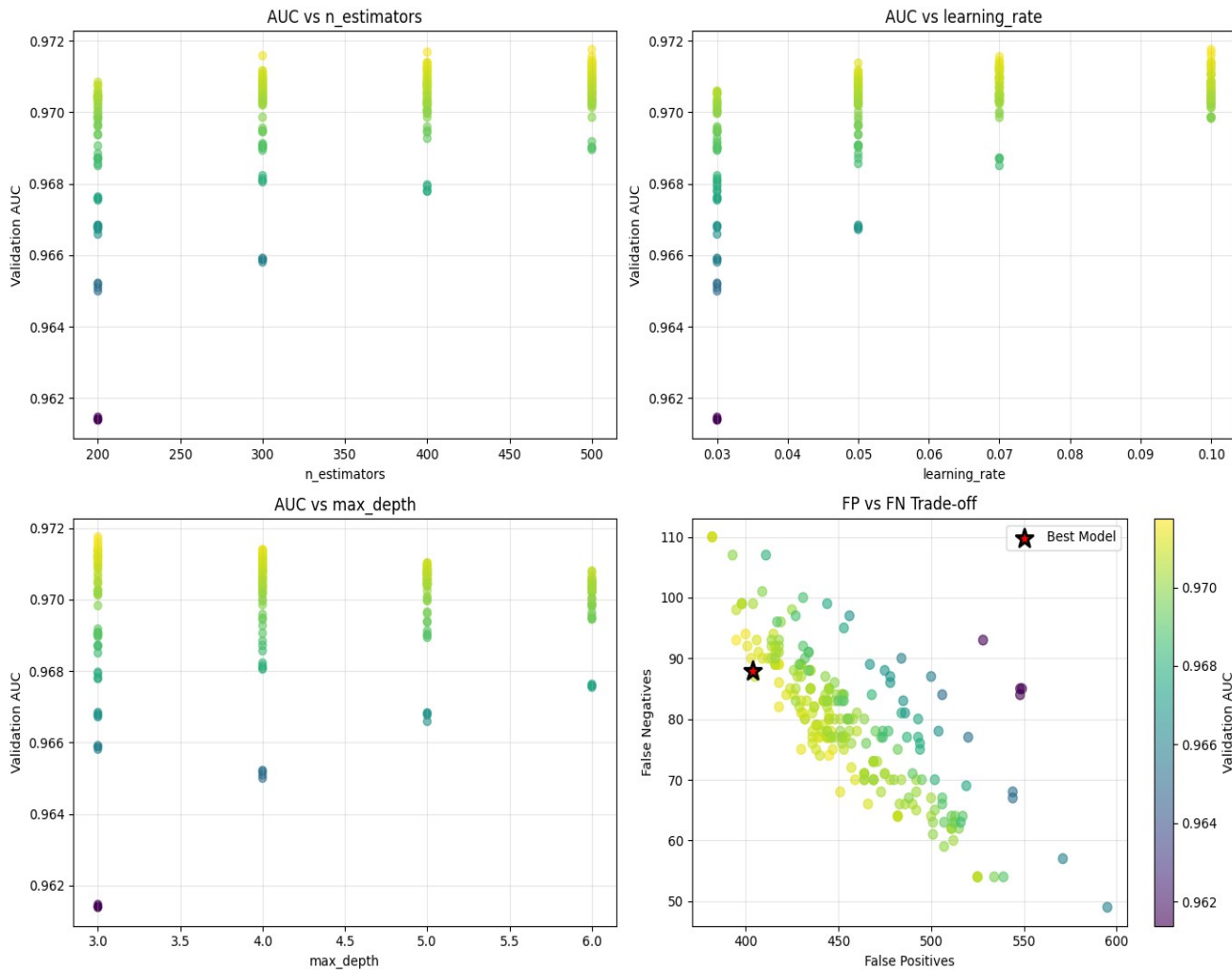
Figures 5.2 – Hyperparameter grid-search results: validation AUC vs. n_estimators, learning rate, max depth, and the FP/FN trade-off of candidate models
