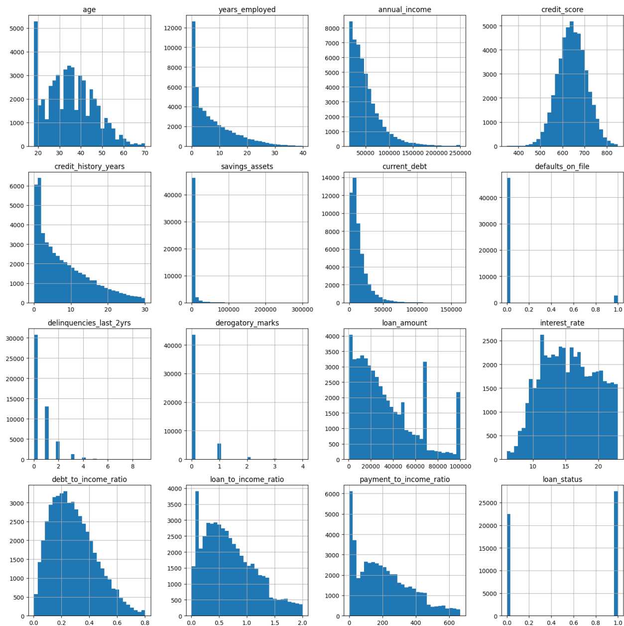
Figure 4.2 – Distributions and histograms of all features
